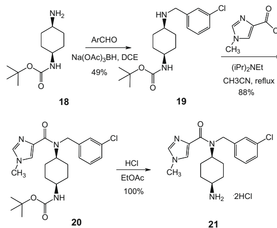
Scheme 2. Preparation of HTS lead compound 21 .
