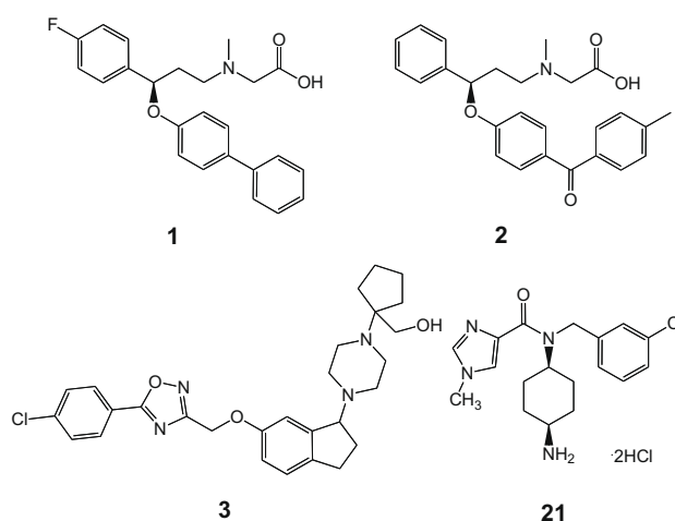
Figure 1. GlyT1 inhibitors discussed above.
