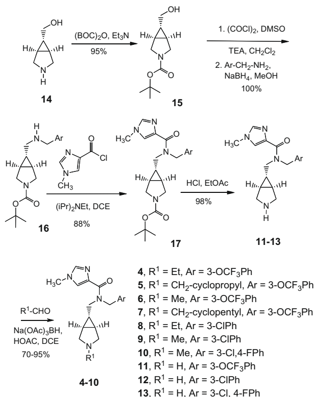
Scheme 1. Preparation of compounds 4 – 17 .
